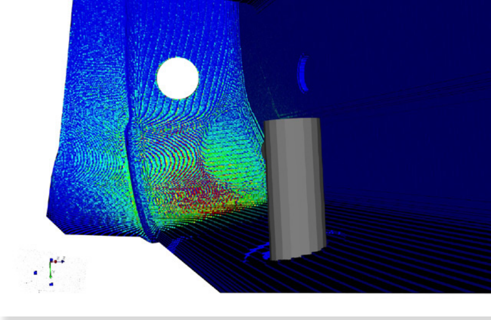
Spray Wax
